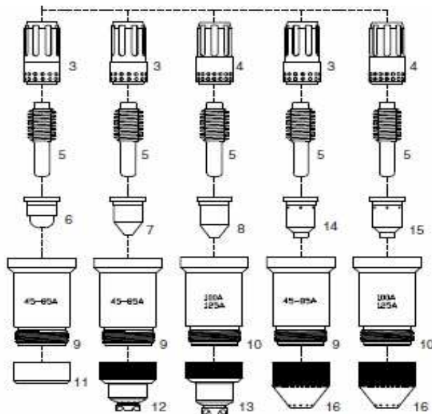
FIGURE 1 - MANUEL & AUTO MT-125 - AT-125
